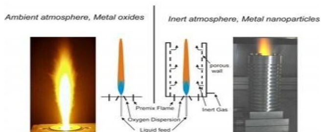
Figure 4. conversion of flame spray synthesis Conventional flame spray synthesis vs Reducing flame spray synthesis
